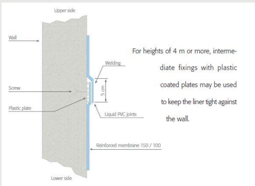
Figure 6: Intermediate mechanical fixation
